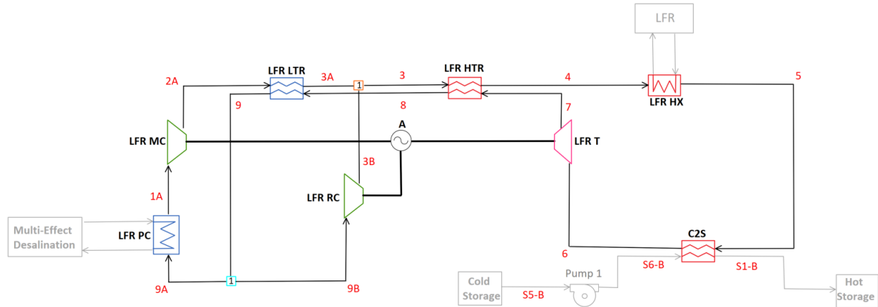
Figure 3.9: Diagram for C-LFR-POST thermal energy storage charging orientation.
