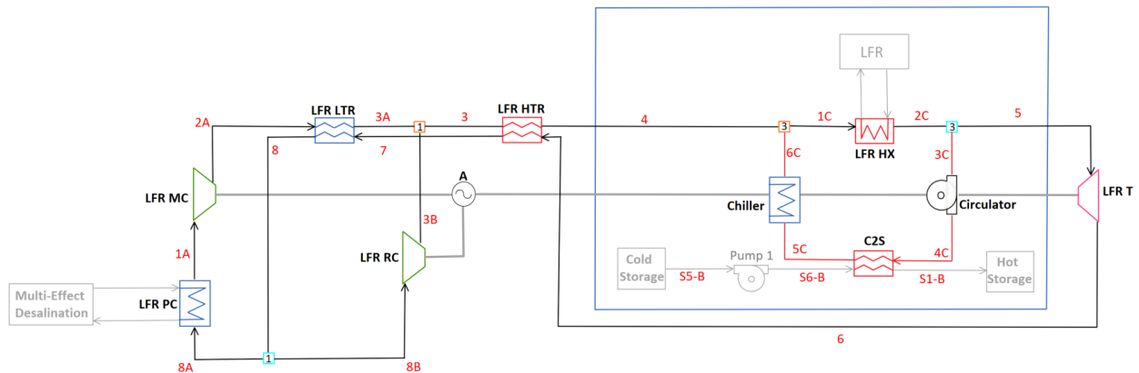
Figure 3.11: Full diagram for C-LFR-CIRC thermal energy storage charging orientation.
