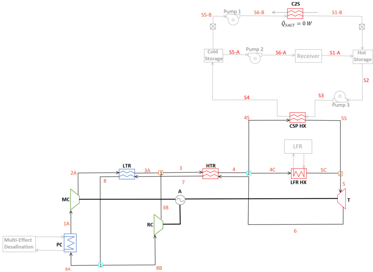
Figure 3.6: Diagram for C-1HTR1T-ON with focus on electricity generation
