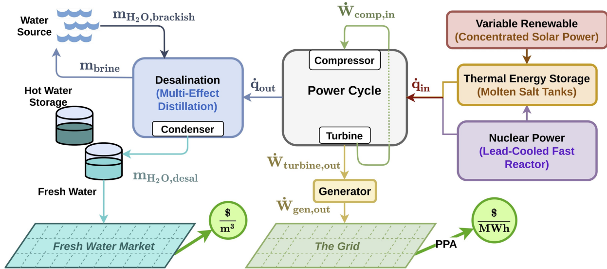
Figure 5.1: IES with the SSRC or s\text{CO}_2 Brayton as primary power cycle. [1]
