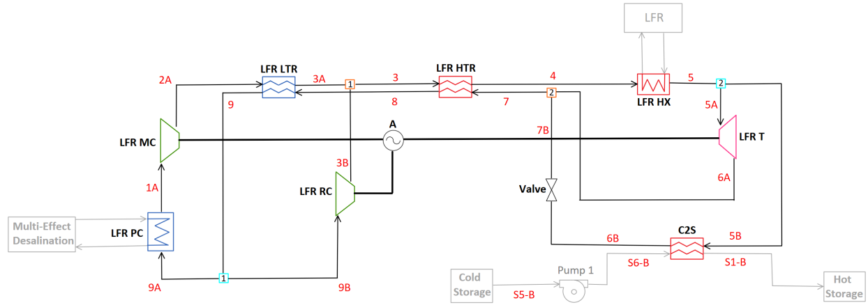
Figure 3.10: Diagram for C-LFR-PAR thermal energy storage charging orientation.
