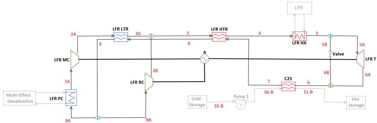
Figure 3.8: Diagram for C-LFR-PRE thermal energy storage charging orientation.
